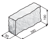
KB 2-10 A GRIND
